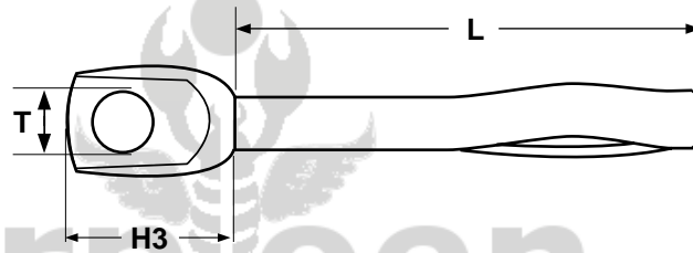
TIE-WIRE HEAD
