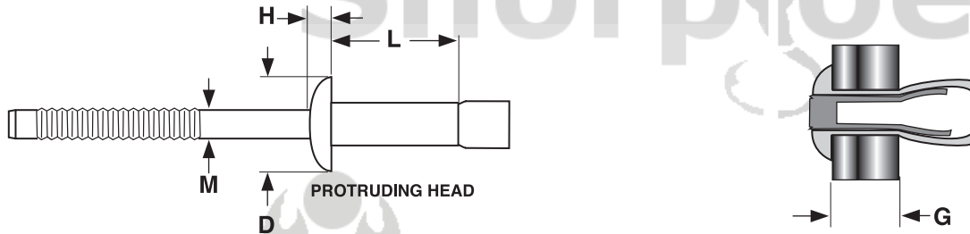
STRUCTURAL RIVETS WITH PROTRUDING HEADS
