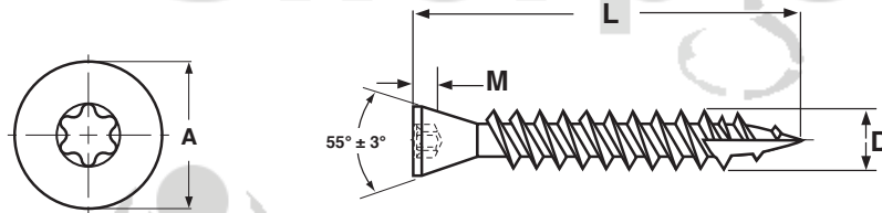
Six-Lobe Drive Trim Head
