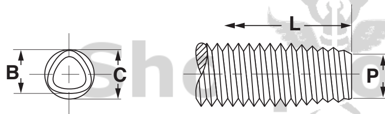
METRIC - TRILOBULAR THREAD ROLLING SCREWS
